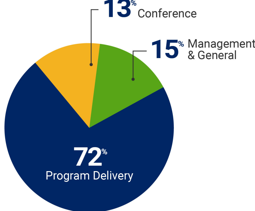
RESNET Expenses 2020
