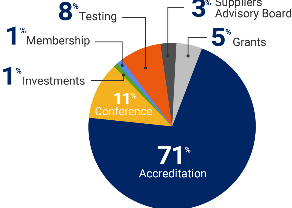
RESNET Revenues 2020
