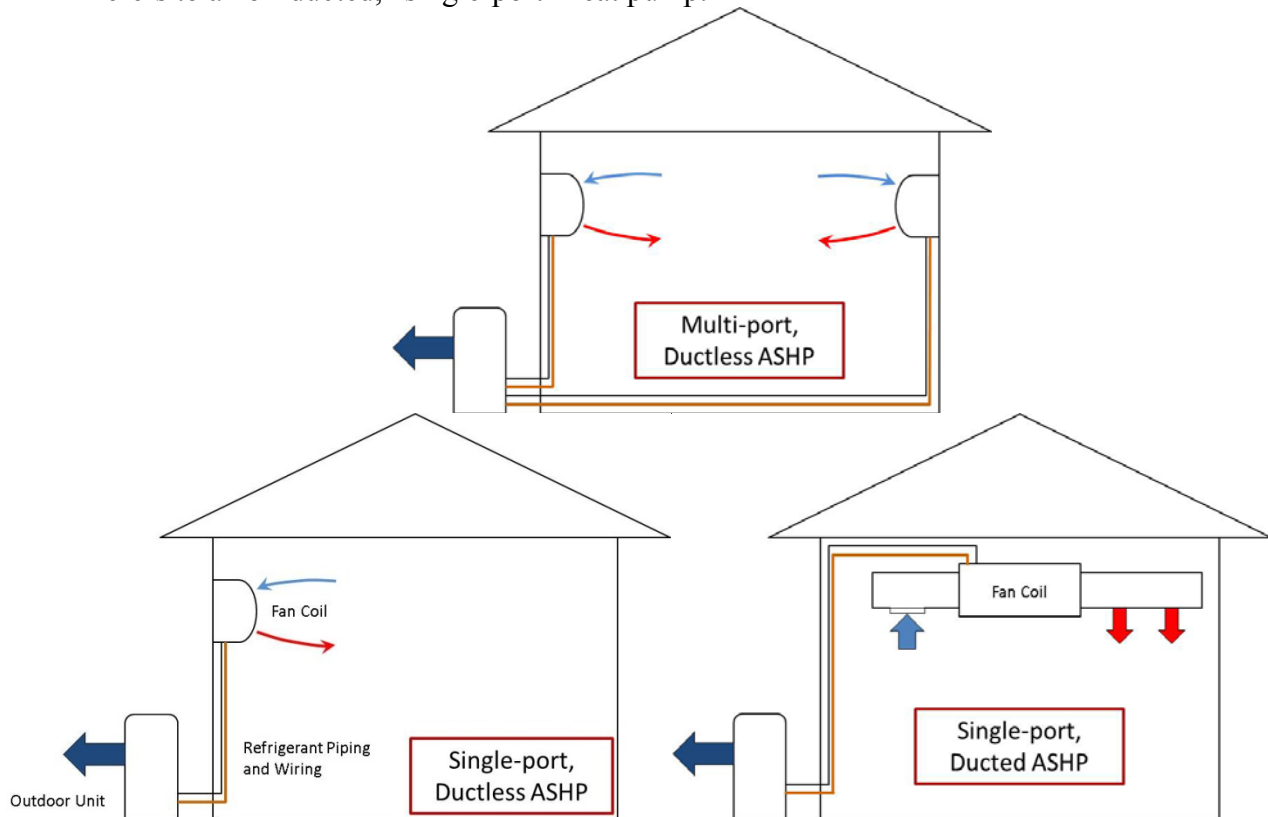
Example schematics of several residential air-source heat pump configurations.
